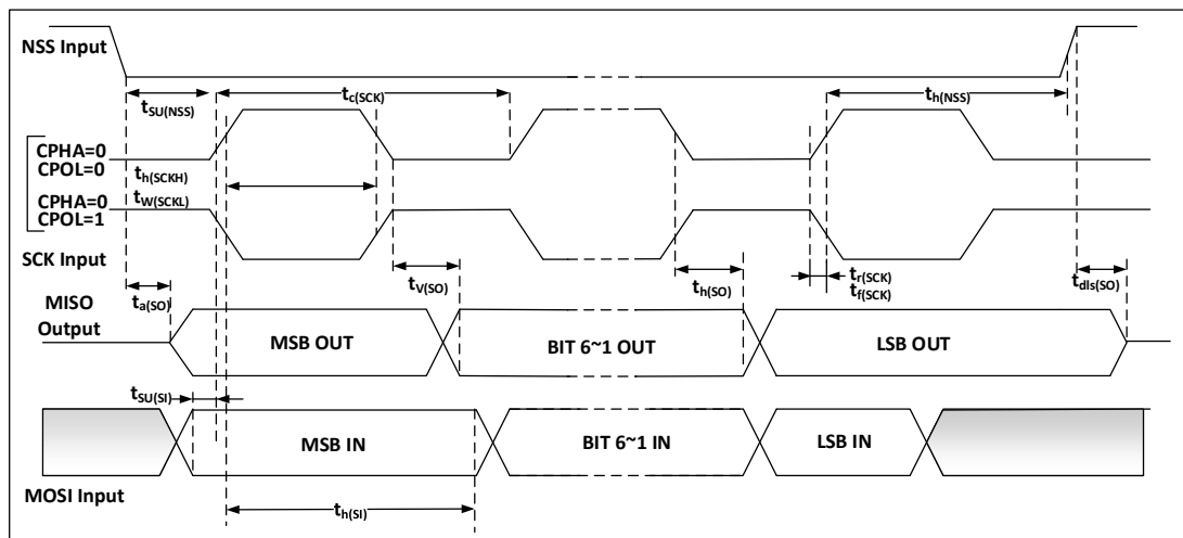
Figure 12 SPI Timing Diagram - Slave Mode and CPHA=0
