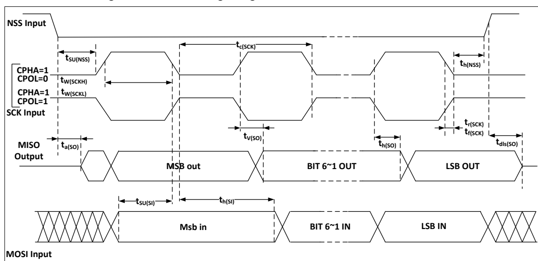
Figure 13 SPI Timing Diagram - Slave Mode and CPHA=1
