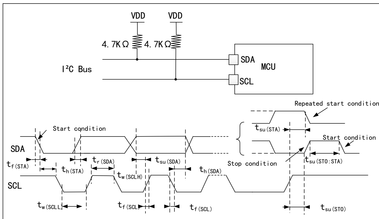
Figure 11 Bus AC Waveform and Measurement Circuit
